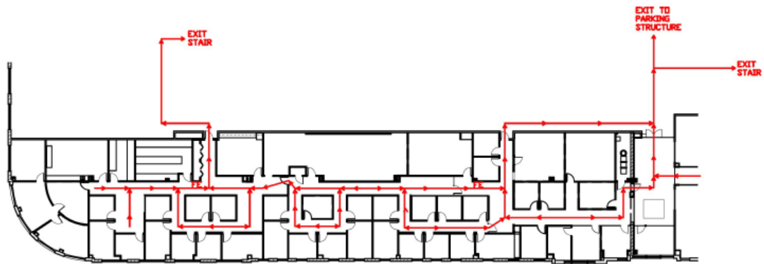
EGRESS PLAN - BAYSHORE WEST FE=Fire Extingulsher AED=Defribrillator
